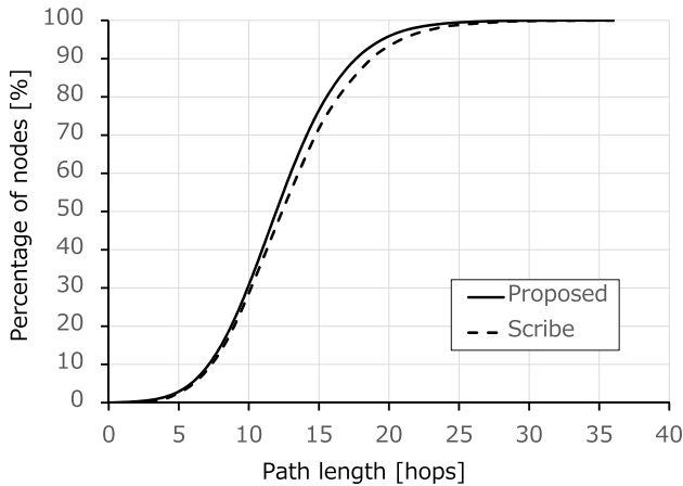
Fig. 11 CDF of path length of pattern α.
