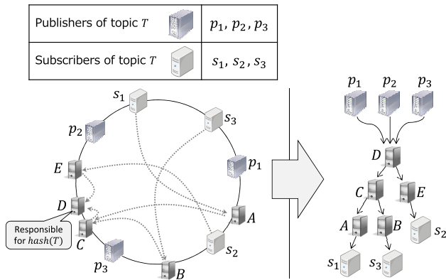
Fig. 2 Topic-based pub/sub by Scribe.
